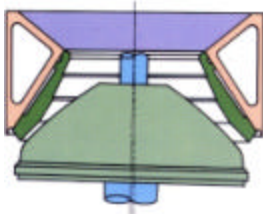
1.CC MODEL For relatively coarse crushing.
